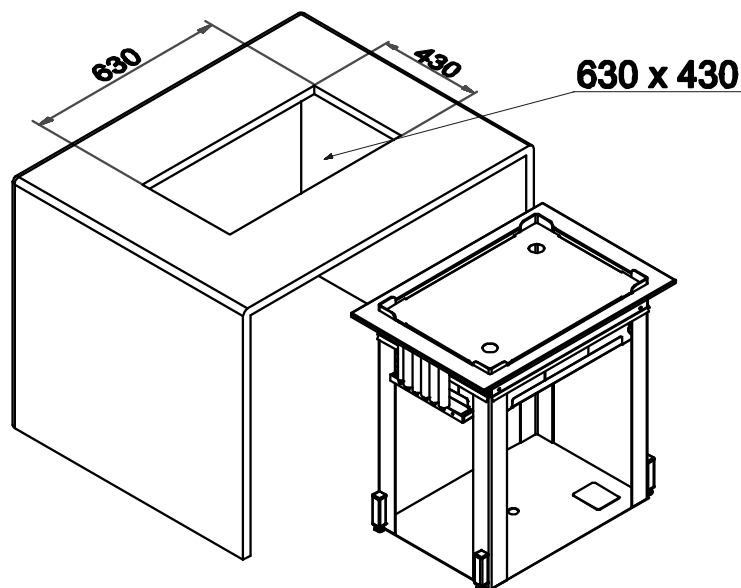
Worktop cut-out EBS-T/53-37
