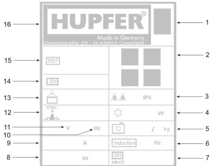
Figure 5 Rating plate
