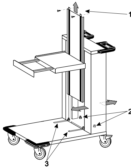
Figure15 Adjust the spring case
