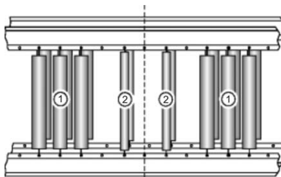
Figure 16 Attachment bar with tension springs (example)
